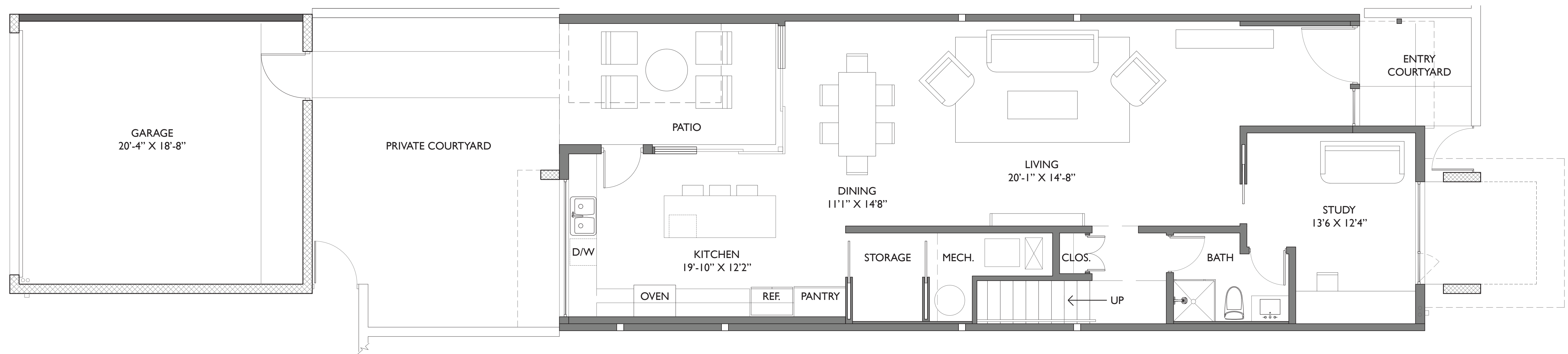
MAIN LEVEL FLOOR PLAN GROSS AREA: 1223 FT 2
