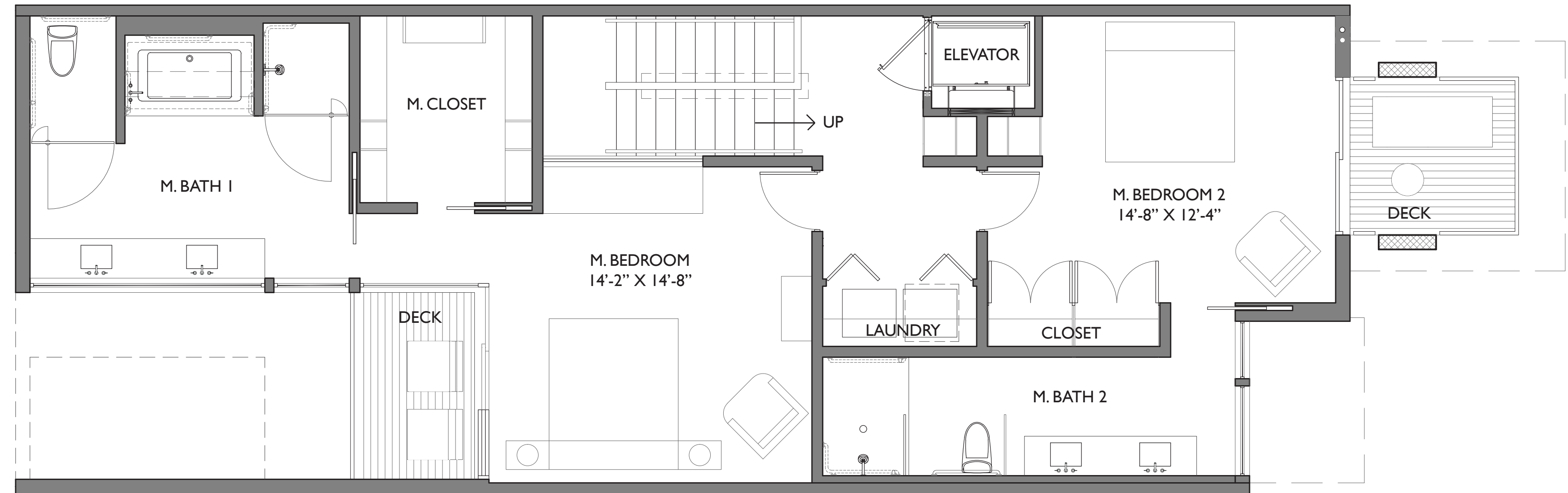
UPPER LEVEL FLOOR PLAN - ELEVATOR GROSS AREA: 1167 FT 2
