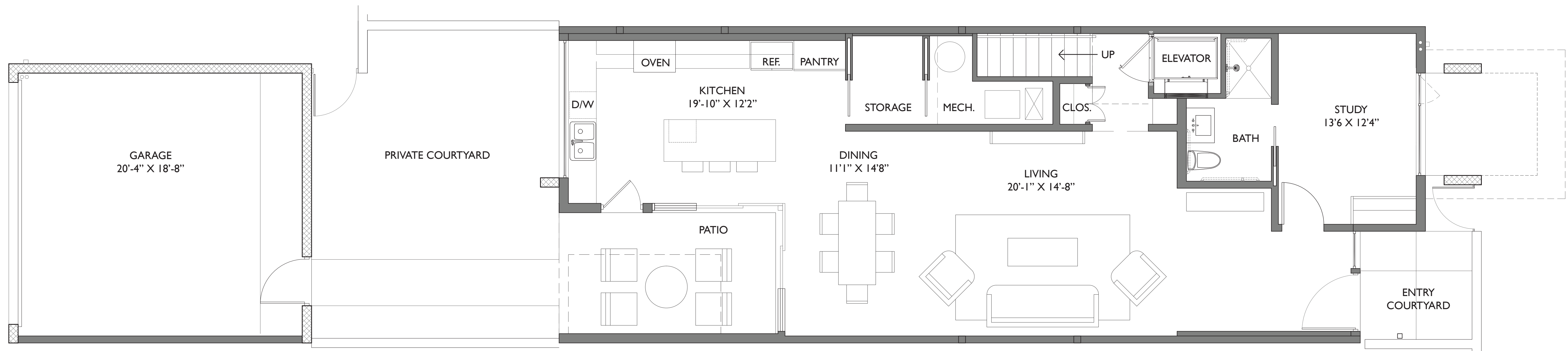
MAIN LEVEL FLOOR PLAN - ELEVATOR GROSS AREA: 1223 FT 2
